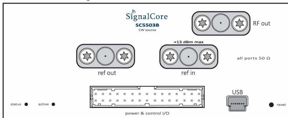
Figure 1. Front view of the SC5503B showing I/O connection locations.
